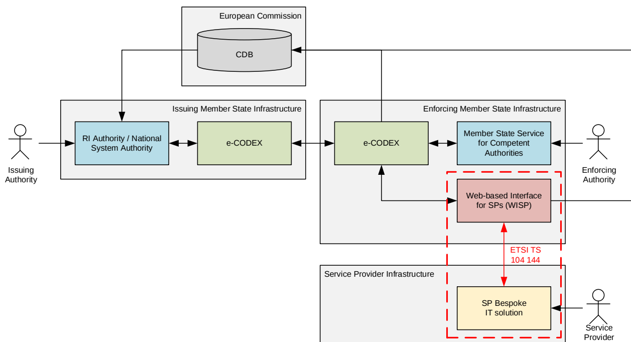
Figure 4.1-1: Wider system of interest
